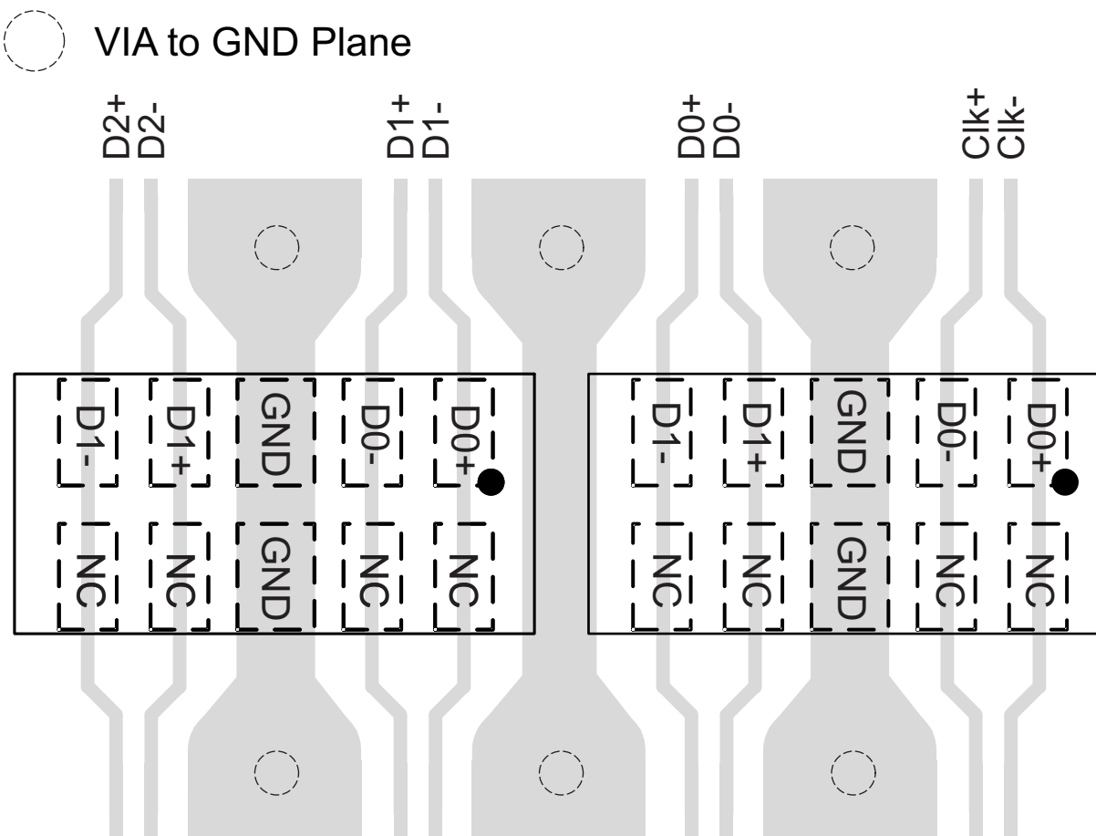
Figure 20. TPD4E05U06 Layout
