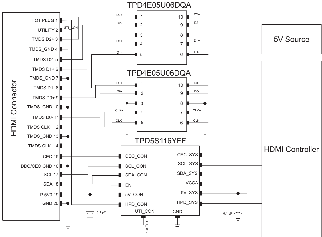
Figure 14. HDMI 1.4 Schematic
