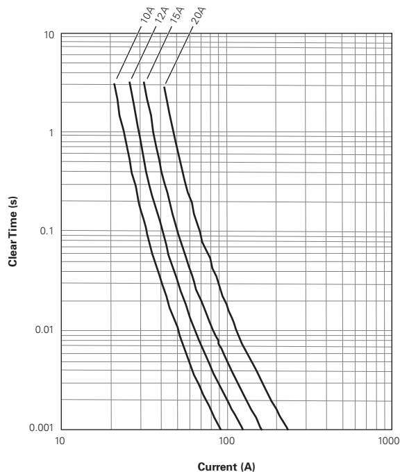
1206SFH Average Time Current Curves
