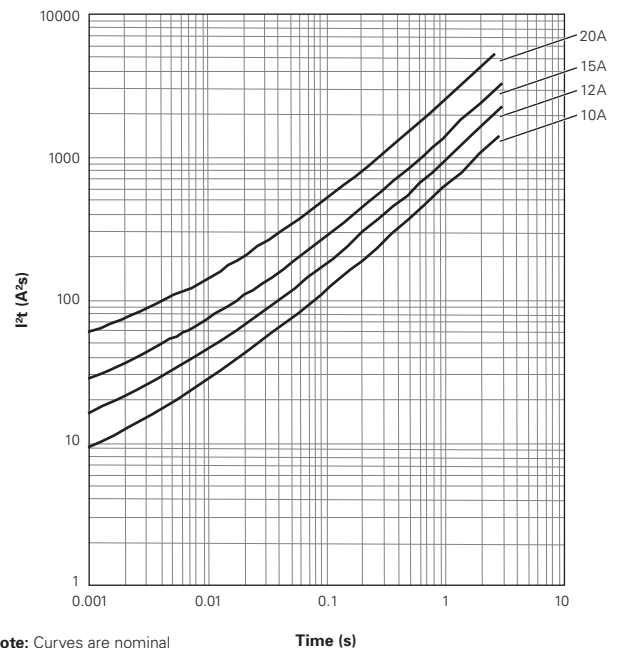
1206SFH I 2 t vs. t Curves
