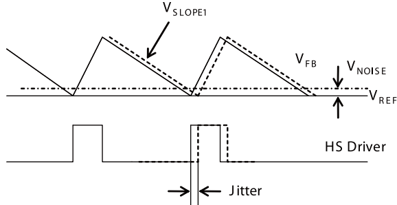
Figure : Jitter in PWM Mode
