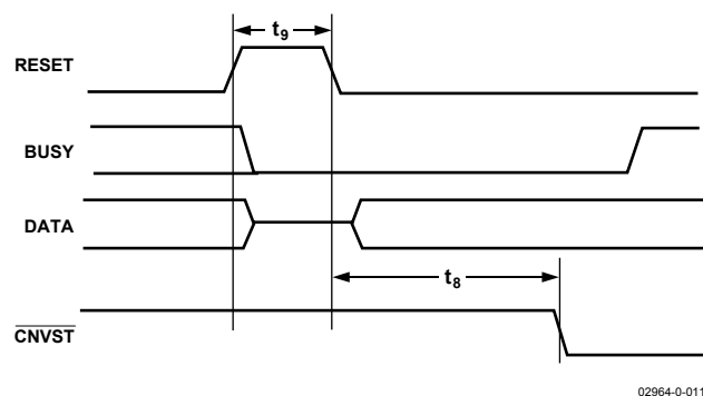
Figure 27. RESET Timing
