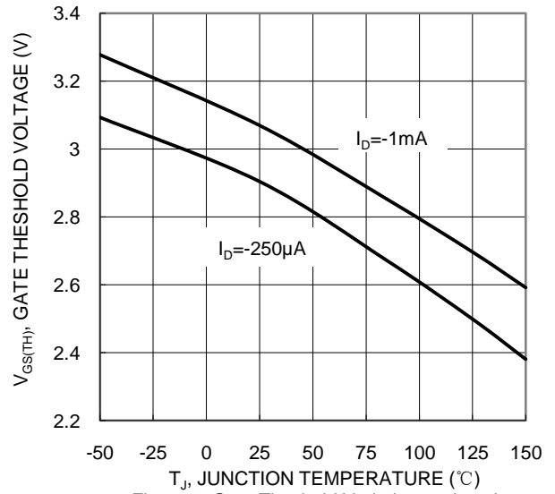
Figure 8. Gate Theshold Variation vs Junction Temperature
