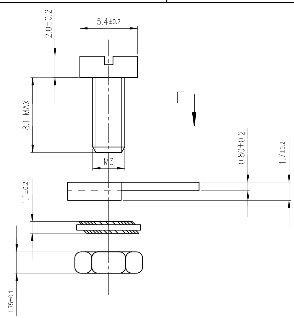
view F
