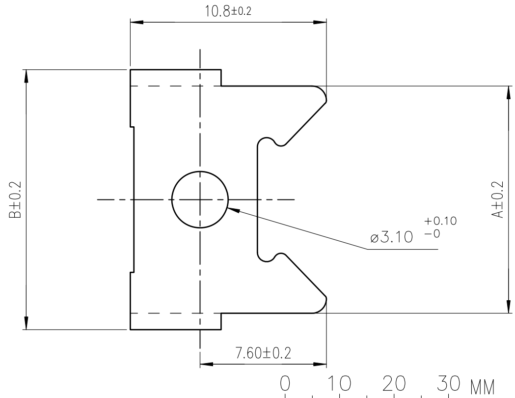
view F
