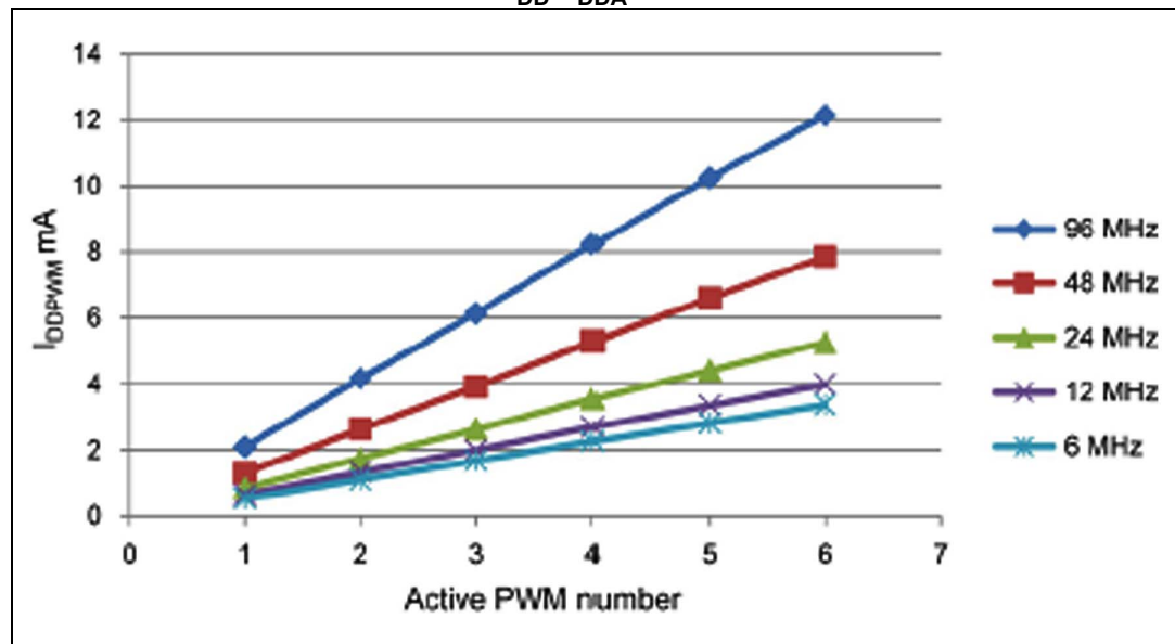
Figure 16. PWM current consumption with f_{\text{SMED}} = \text{PLL } f_{\text{PWM}} = 0.5\text{ MHz} at V_{\text{DD}}/V_{\text{DDA}} = 5\text{ V}
