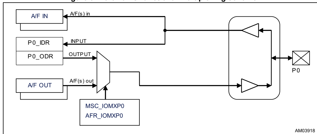
Figure 9. Port P0 I/O functional multiplexing scheme
