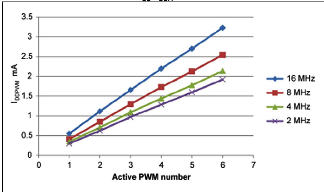
Figure 18. PWM current consumption with f_{SMED} = HSI f_{PWM} = 0.5 MHz at V_{DD}/V_{DDA} = 5 V
