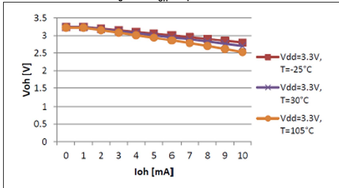
Figure 25. V_{OH} fast pad at 3.3 V
