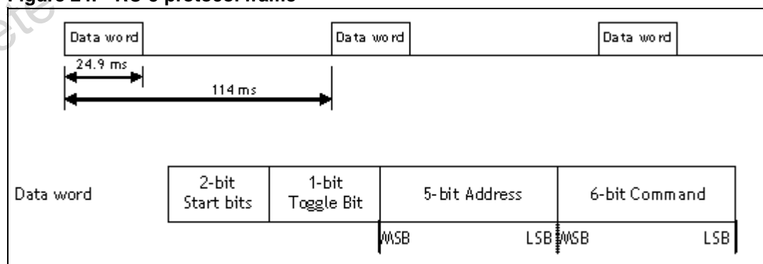
Figure 24. RC-5 protocol frame
