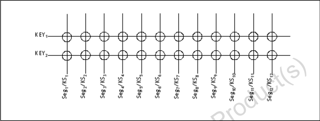
Figure 10. Key matrix (12 x 2 configuration) and key-input data storage RA
