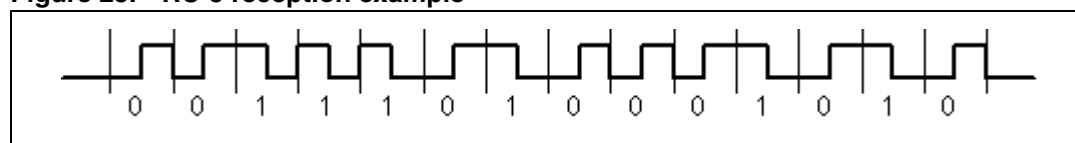
Figure 25. RC-5 reception example
