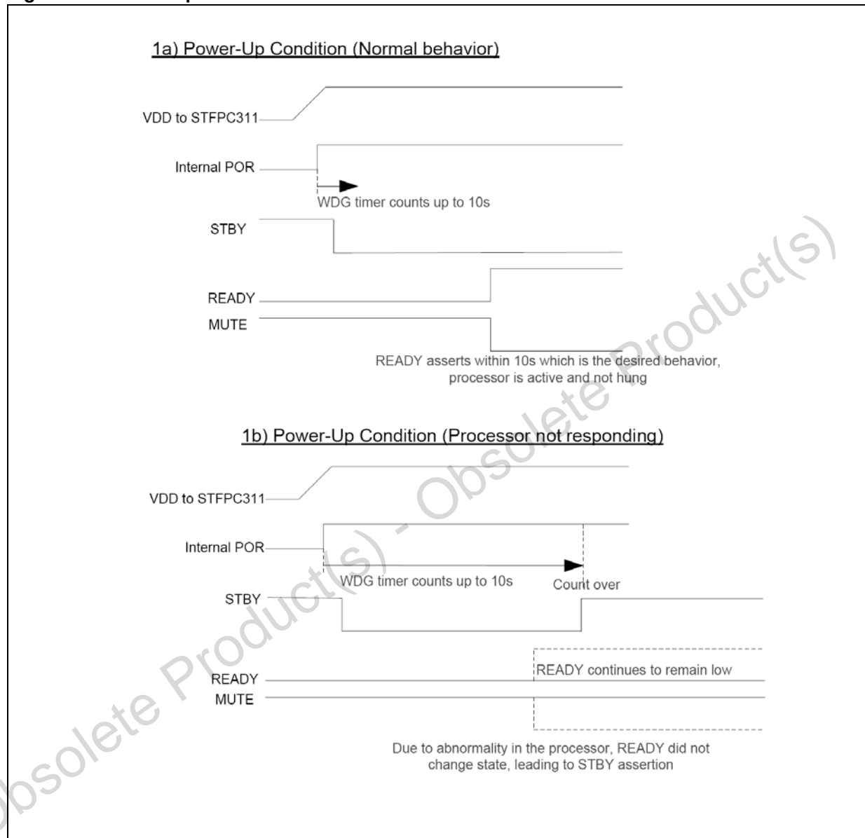
Figure 3. Power-up condition
