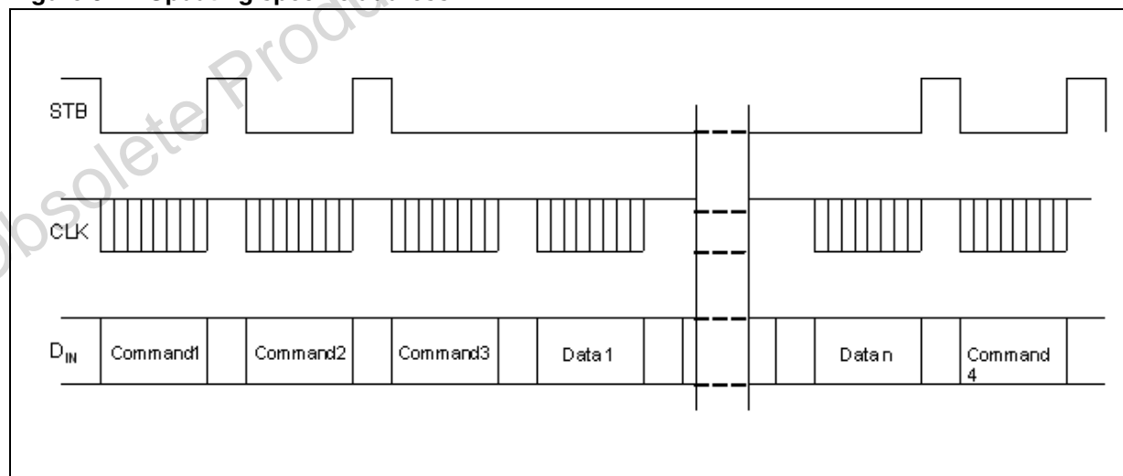
Figure 34. Updating specific address
