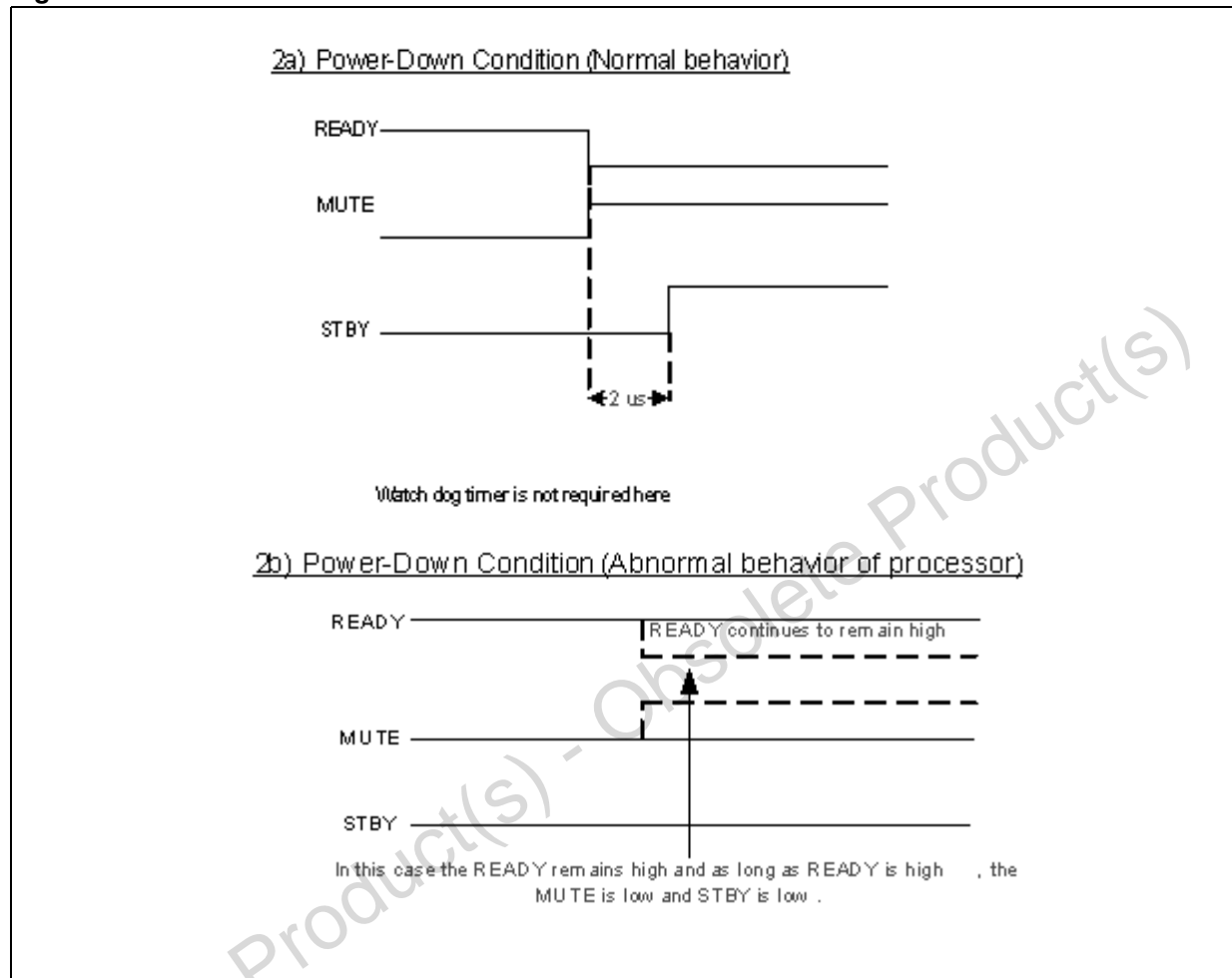
Figure 4. Power-down condition
