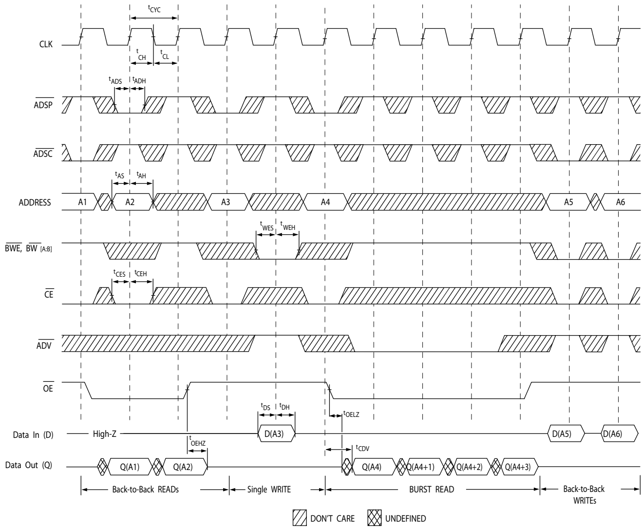
Figure 5. Read/Write Timing [22, 23, 24]
