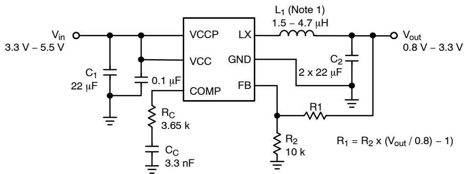
Figure 2. NCP1599 Application Circuit
