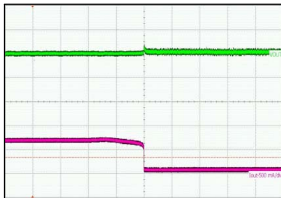
( V_{IN} = 5\text{ V} , I_{LOAD} = 100\text{ mA} , L = 2.2\ \text{H} , C_{OUT} = 2 \times 22\ \mu\text{F} ) Upper Trace: Output Dynamic Voltage, 100 mV/div Lower Trace: Output Current, 500 mA/div Time Scale: 200 \mu\text{s}/\text{div}
