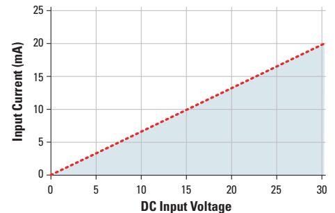
Input Current vs Input Voltage "T" Option - Low Voltage Output
