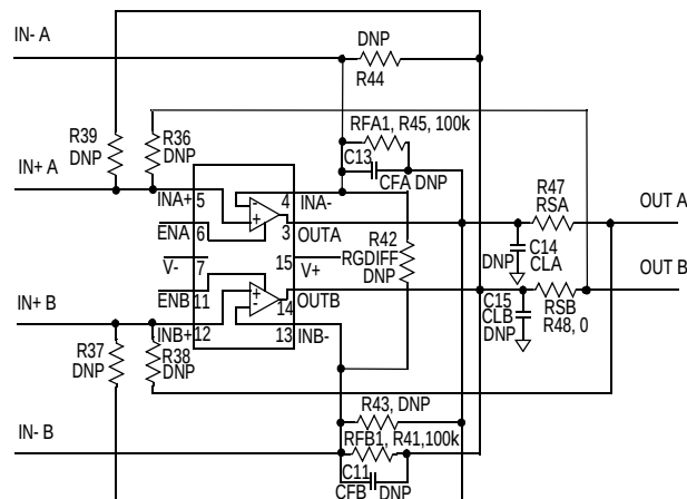
FIGURE 5. OPTIONAL COMPONENTS
