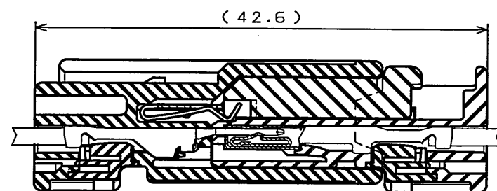
MATED CONDITION(REF.) 組込後状態図(参考)
