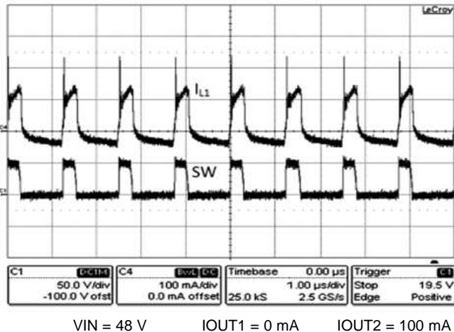
Figure 22. Steady State Waveform
