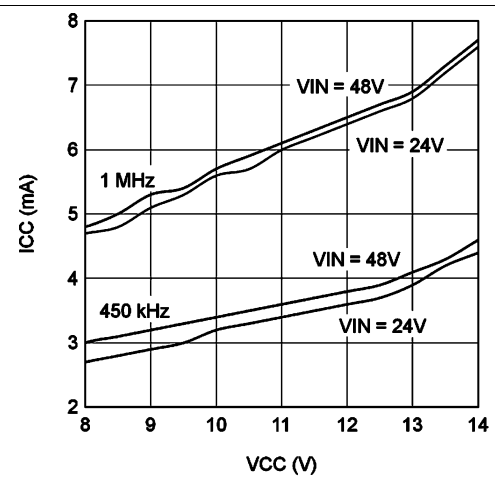
Figure 4. I_{CC} vs External V_{CC}
