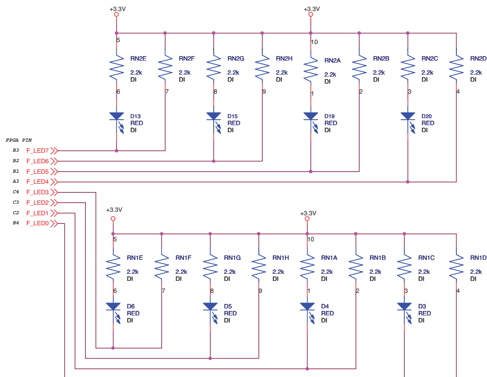
Figure 4. FPGA LEDs
