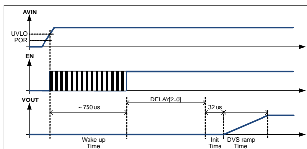
Figure 34. Initial Power Up Sequence
