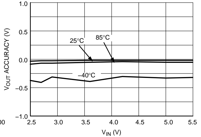
Figure 13. V_{OUT} Accuracy vs V_{IN} and Temperature V_{OUT} = 1.15\text{ V} , I_{LOAD} = 2.0\text{ A}
