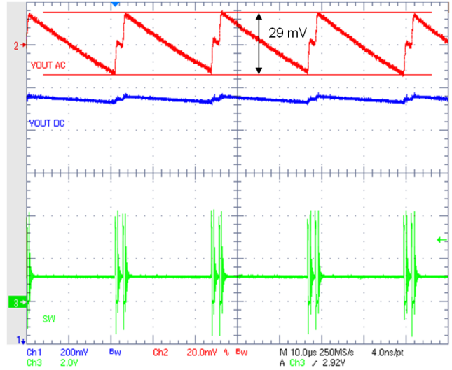
Figure 25. PFM Ripple
