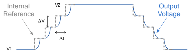
Figure 38. DVS in Forced PWM Mode Diagram
