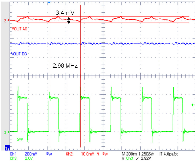
Figure 24. PWM Ripple
