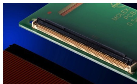
Standard Cable Type, 2.50mm Height (502790 Series)
