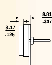
Window Mount Side View
