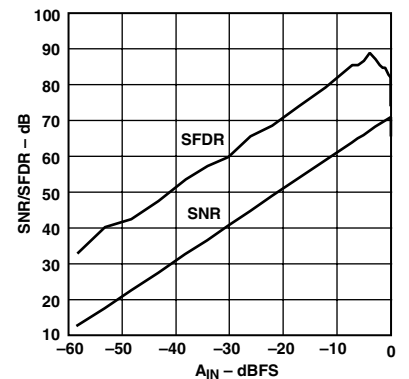
TPC 18. SNR/SFDR vs. A_{IN} (Input Amplitude) ( f_{IN} = 1.5\text{ MHz} , Input Span = 2 V p-p, V_{CM} = 2.5\text{ V} )
