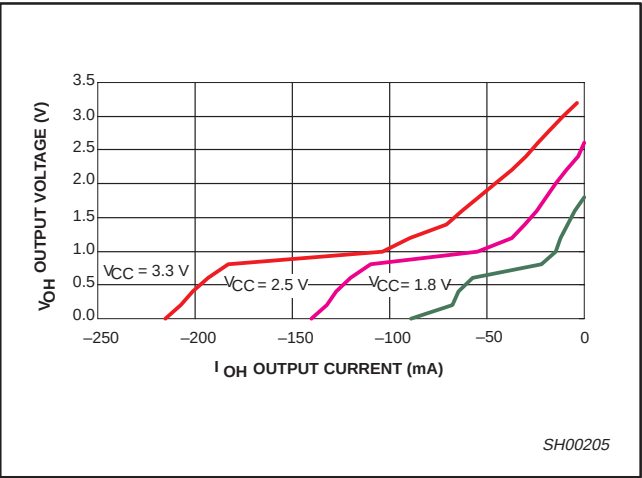
Figure 2. Output voltage (V OH ) vs. output current (I OH )
