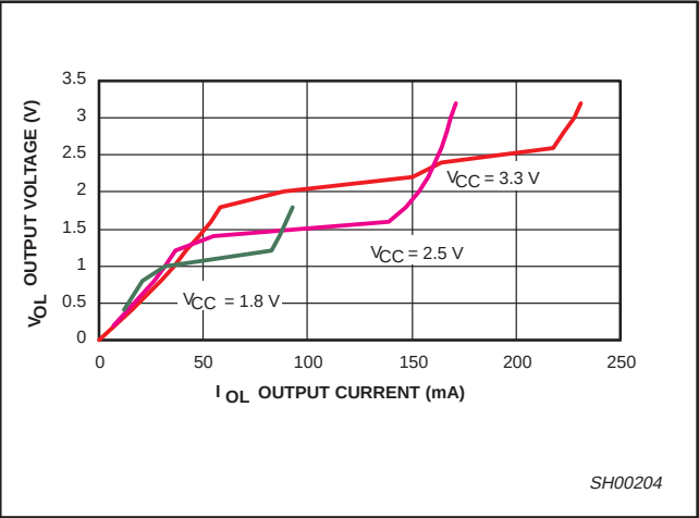
Figure 1. Output voltage (V OL ) vs. output current (I OL )
