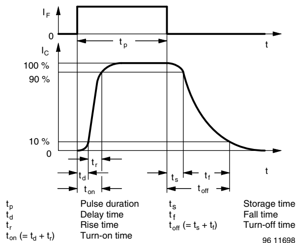
Fig. 4 - Switching Times
