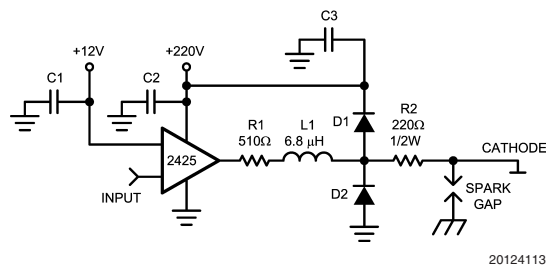
FIGURE 13. One Channel of the LM2425 with the Recommended Application Circuit
