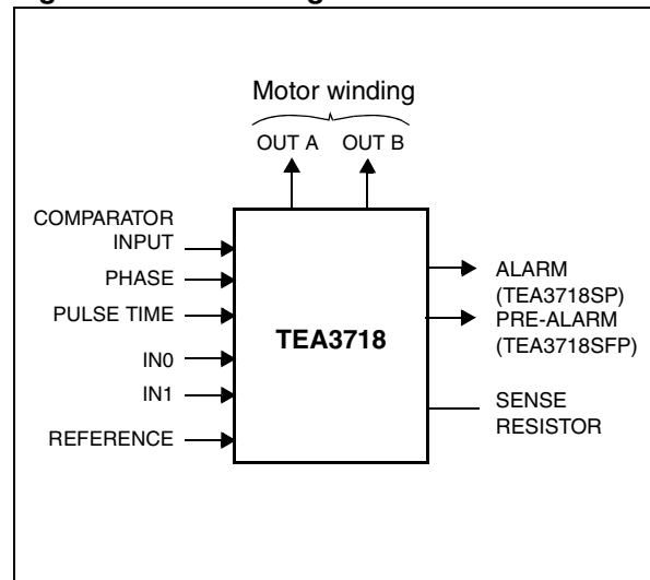
Figure 1. Block diagram
