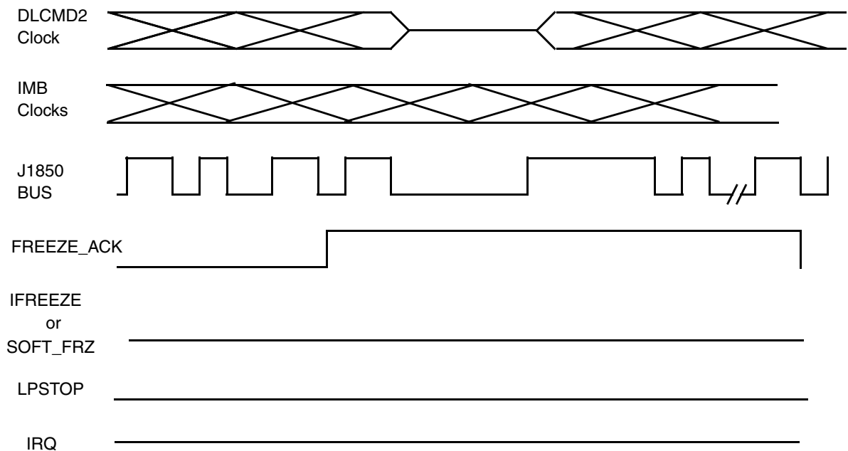
Figure 15-14. DEBUG Power Mode (IFREEZE or SOFT_FRZ)
