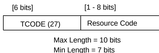
Figure 23-31. Program Trace Full Message Format
