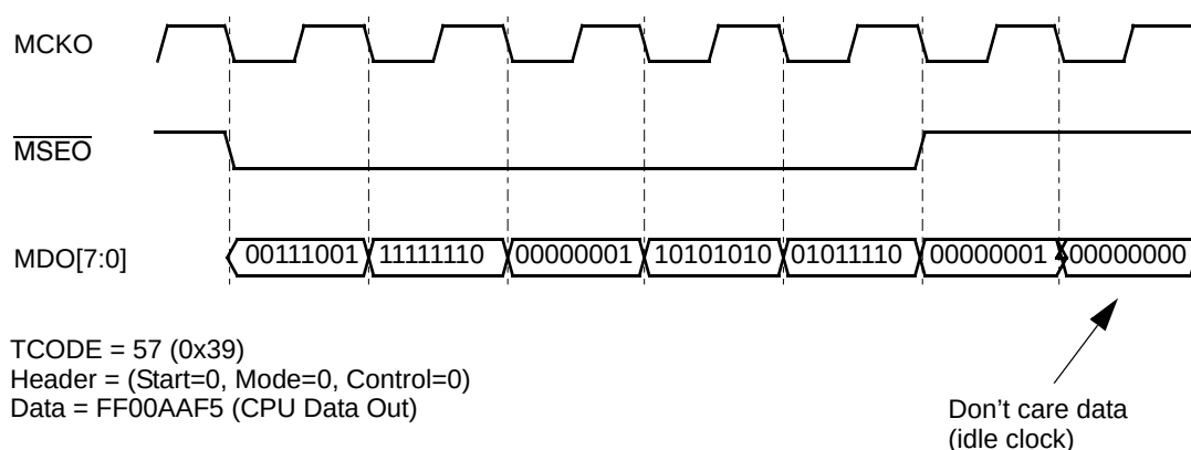
Figure 23-88. DSDO Data Message (CPU Data Out)
