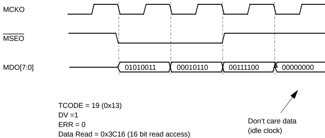
Figure 23-67. Upload/Download Information Message
