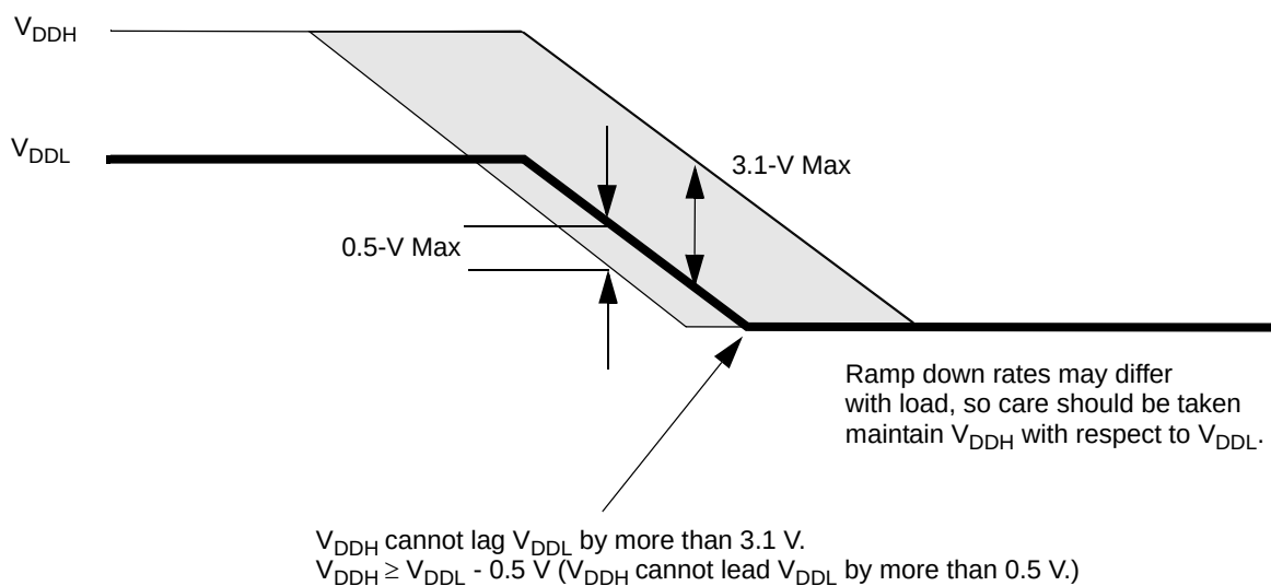
Figure F-3. Option A Power-Down Sequence Without Keep-Alive Supply
