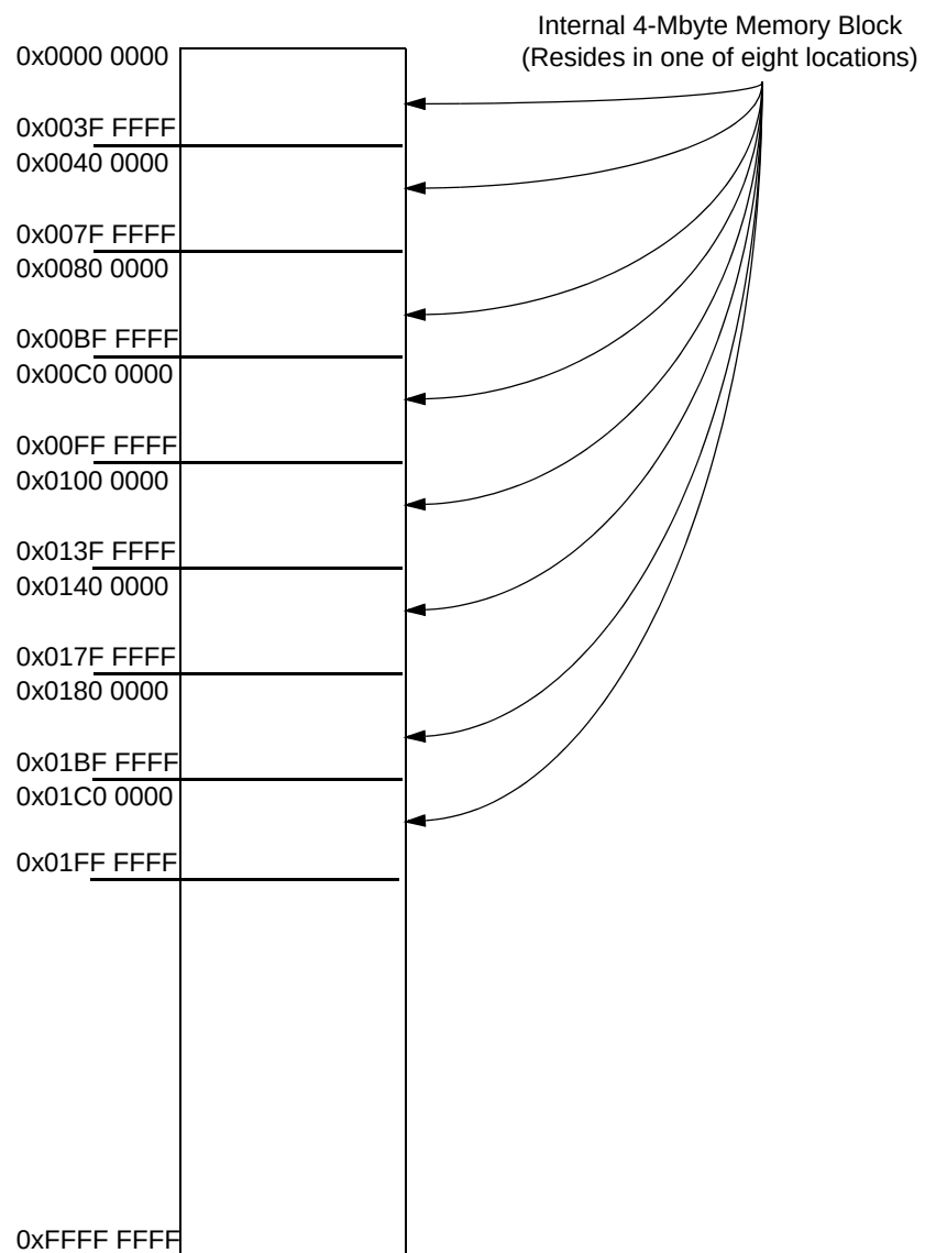
Figure 1-2. Memory Map
