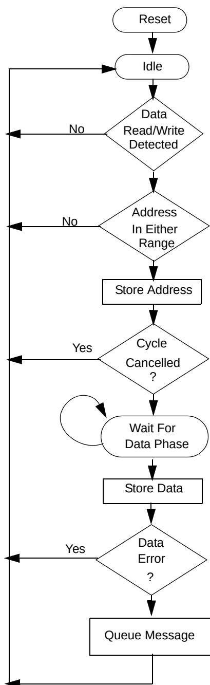
Figure 23-48. Data Trace Flow Diagram for Non-Pipelined Access
