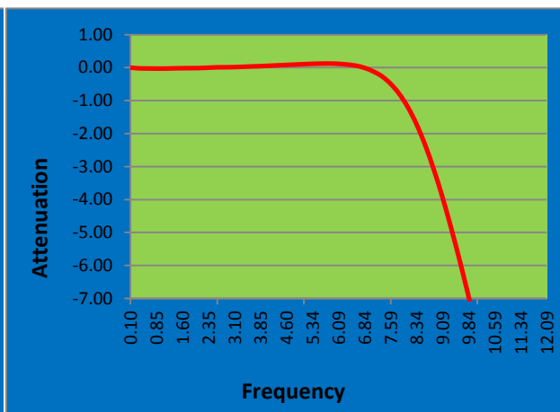
Figure 4. SD Flatness
