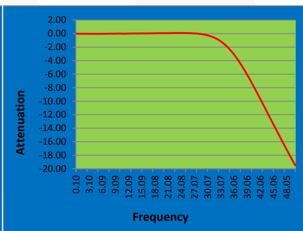
Figure 6. HD Flatness
