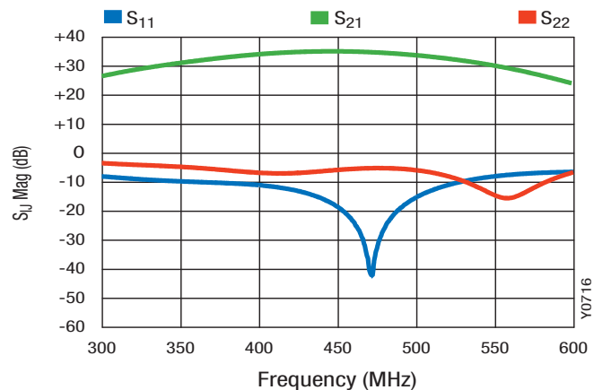
Figure 24. S-Parameters vs Frequency
