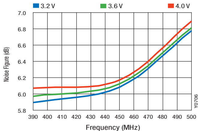
Figure 14. Noise Figure vs Frequency Across VCC
