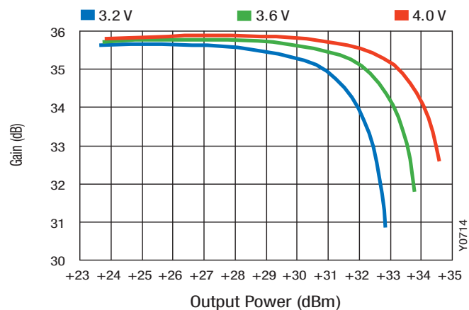
Figure 22. Gain vs Output Power Across VCC
