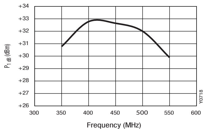
Figure 26. P1dB vs Frequency
