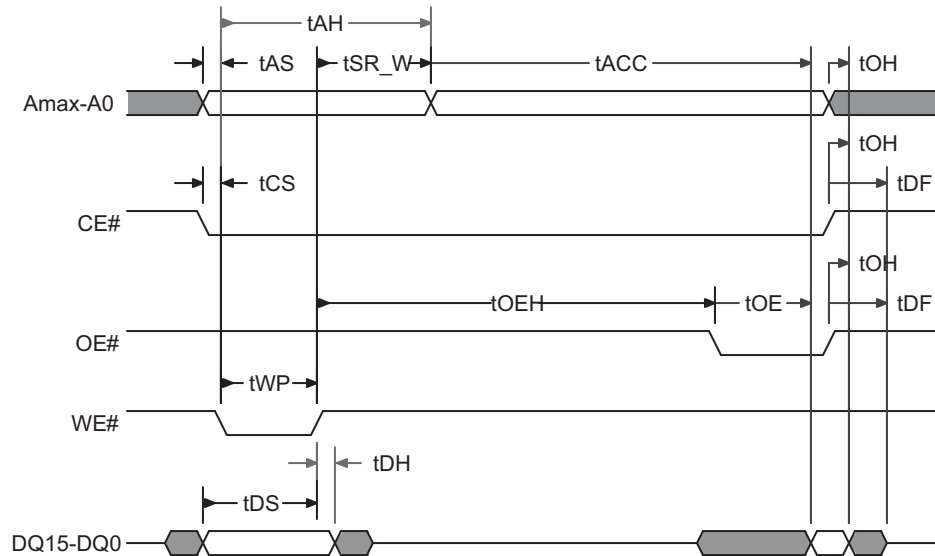
Figure 10.10 Write to Read ( t_{ACC} ) Operation Timing Diagram
