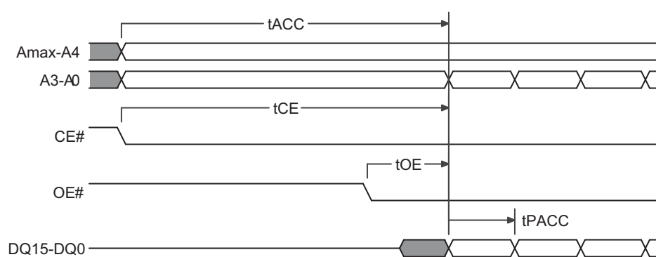
Figure 10.7 Page Read Timing Diagram
