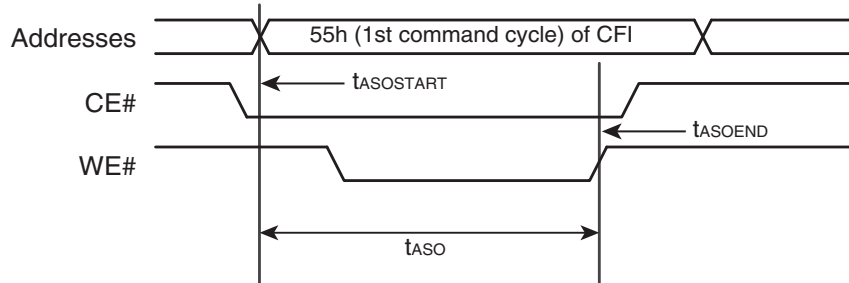
Figure 10.16 ASO Entry Timing
