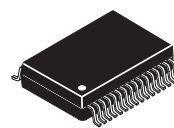
EK SUFFIX (PB-FREE) 98ARL10543D 32-PIN SOICW-EP
