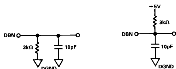
Figure 3. Load Circuits for Access Time Tests (t 12 )
