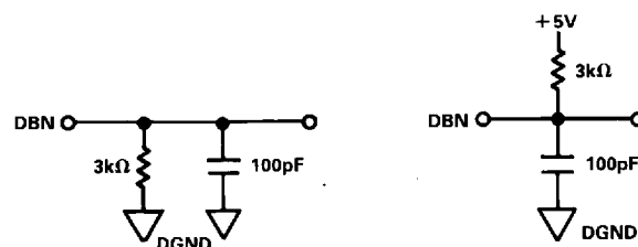
Figure 3. Load Circuits for Access Time Tests (t 12 )
