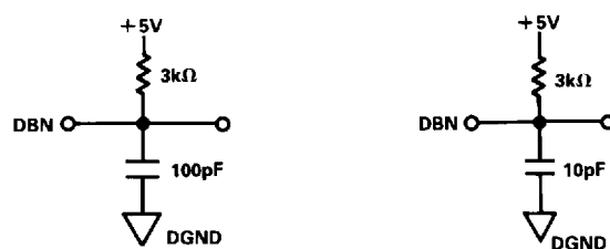
Figure 4. Load Circuits for Output Float Delay (t 13 )
