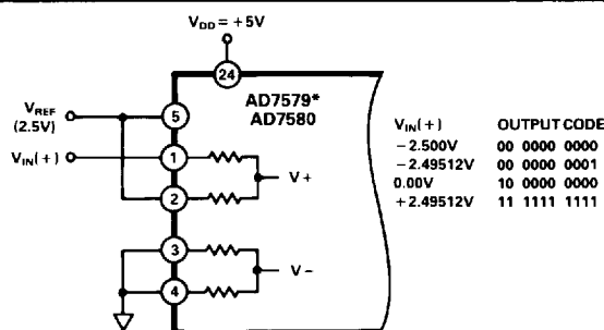
Figure 16. Single-Ended Bipolar Operation, -2.5V to +2.5V
