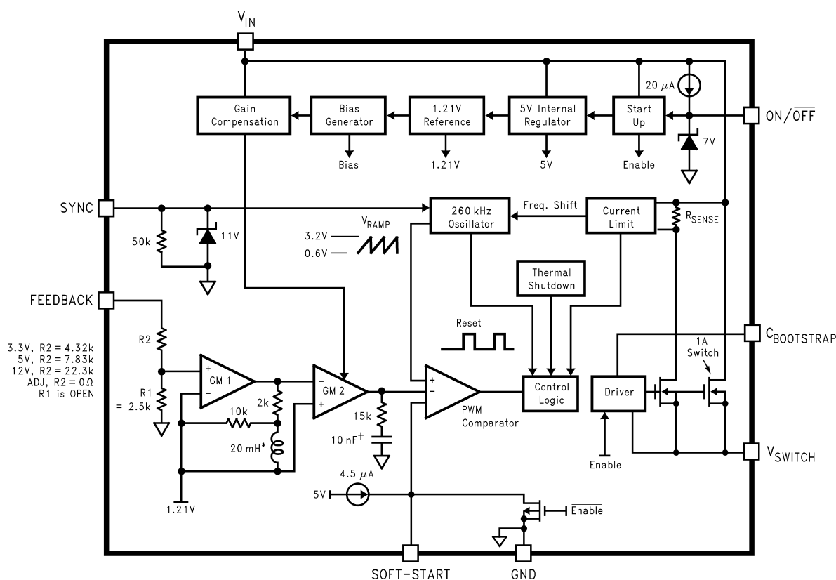
Figure 17. Block Diagram
