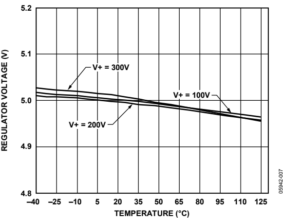
Figure 20. Regulator Voltage vs. Temperature (High Voltage Operation)
