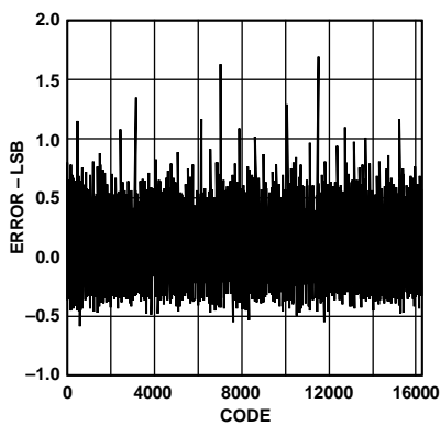
Figure 16. Typical DNL
