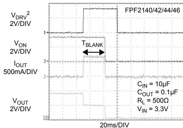
Figure 22. T_{BLANK} Response
