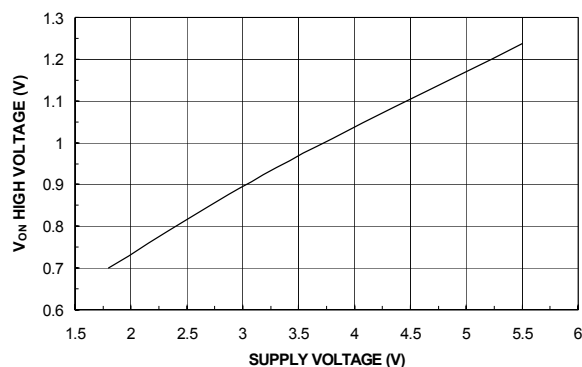
Figure 3. V ON High Voltage vs. Input Voltage
