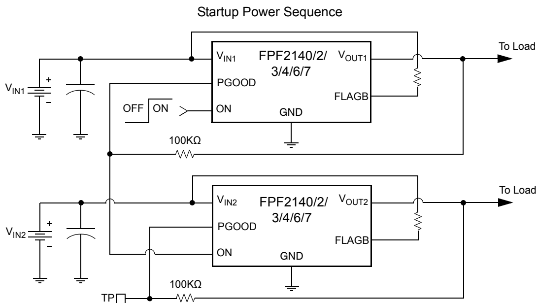
Power good function in sequential startup. No battery is loaded to the output
