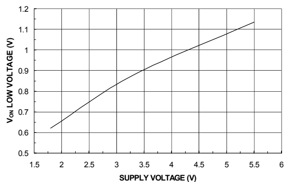
Figure 4. V ON Low Voltage vs. Input Voltage
