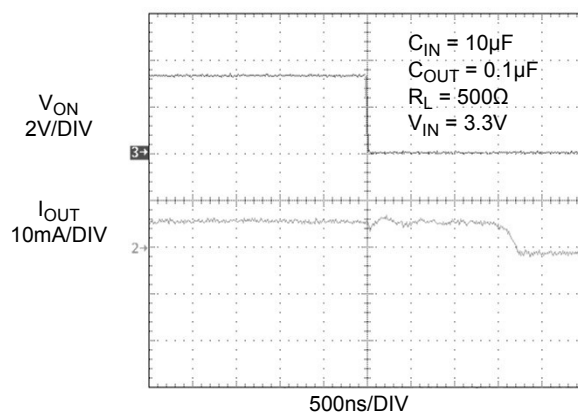
Figure 16. t dOFF Response
