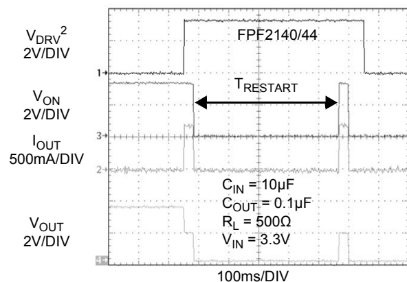
Figure 23. T_{RESTART} Response
