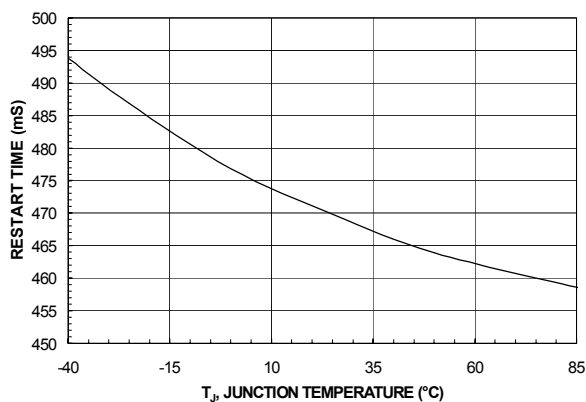
Figure 14. T RESTART vs. Temperature
