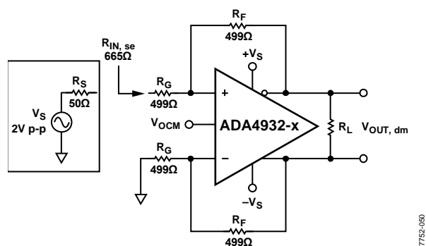
Figure 59. Calculating Single-Ended Input Impedance, R_{IN}
