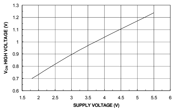
Figure 3. V ON High Voltage vs. Input Voltage
