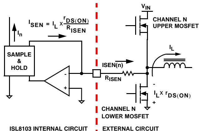
FIGURE 5. ISL8103 INTERNAL AND EXTERNAL CURRENT-SENSING CIRCUITRY FOR CURRENT BALANCE
