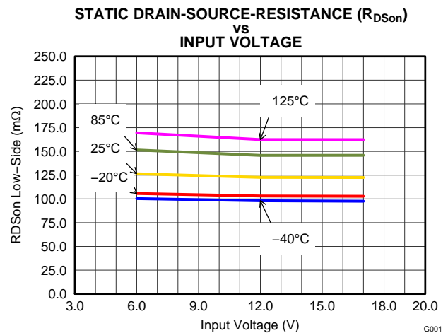
Figure 20. Low-Side Switch
