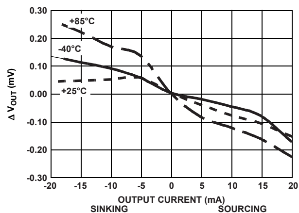
FIGURE 11. LOAD REGULATION
