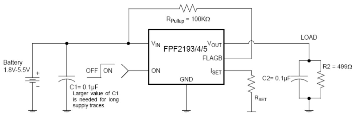
Figure 28. Typical Application
