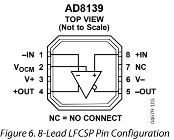
Figure 6. 8-Lead LFCSP Pin Configuration
