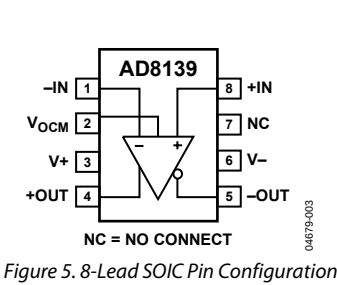
Figure 5. 8-Lead SOIC Pin Configuration
