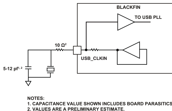
Figure 7. External USB Crystal Connection
