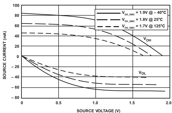
Figure 62. Driver Type C Current (1.8 V V_{DD\_DMC} )
