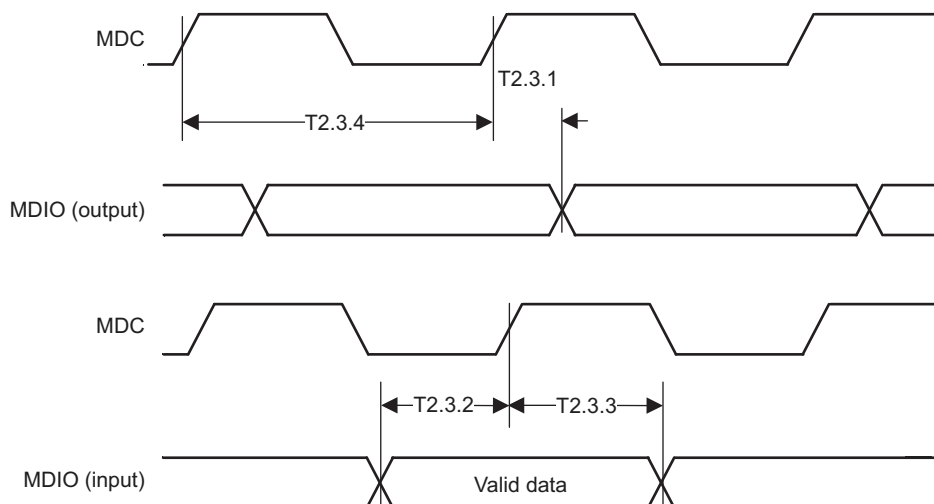
Figure 3-4. MII Serial Management Timing
