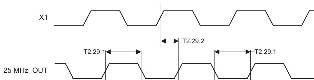
Figure 3-30. 25 MHz_OUT Timing
