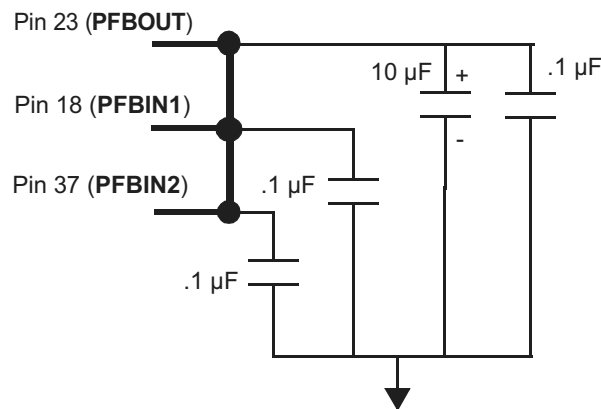
Figure 7-3. Power Feedback Connection
