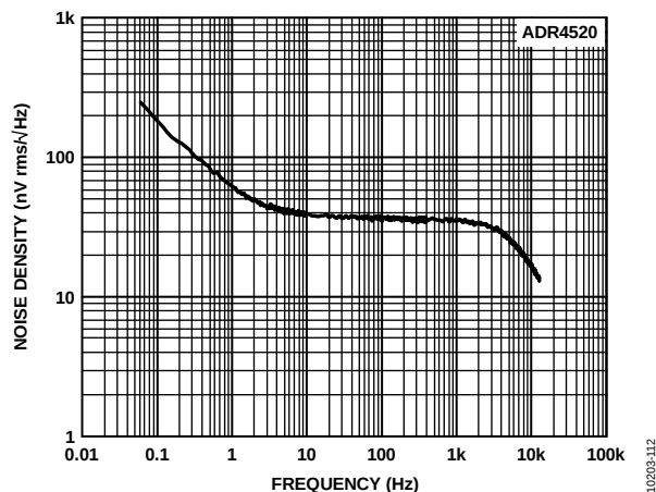
Figure 12. ADR4520 Output Noise Spectral Density
