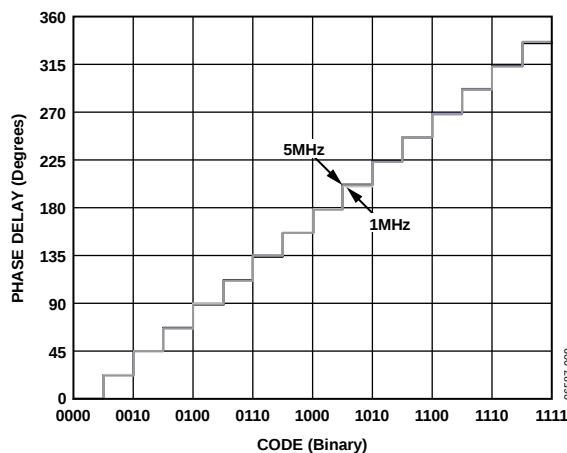
Figure 10. Representative Phase Delay vs. Binary Phase Select Code at 1 MHz and 5 MHz; Ch 3 and Ch 4 Are Displayed with Respect to Ch 1
