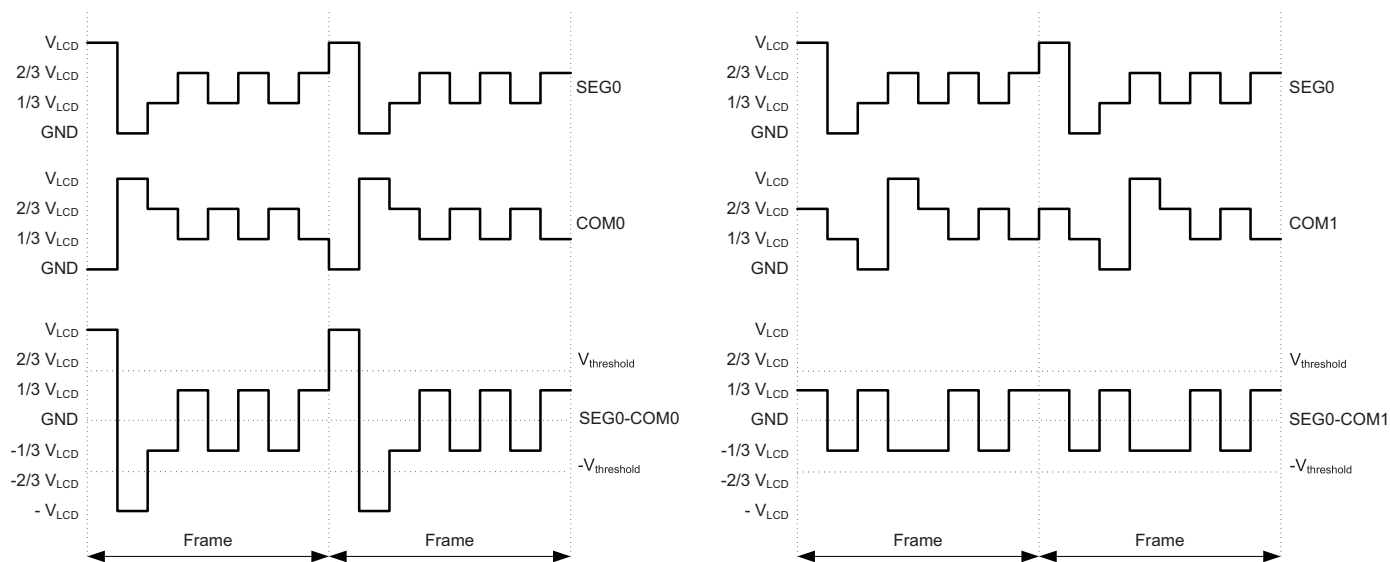
Figure 39-7. Driving a LCD With Four Common Lines
