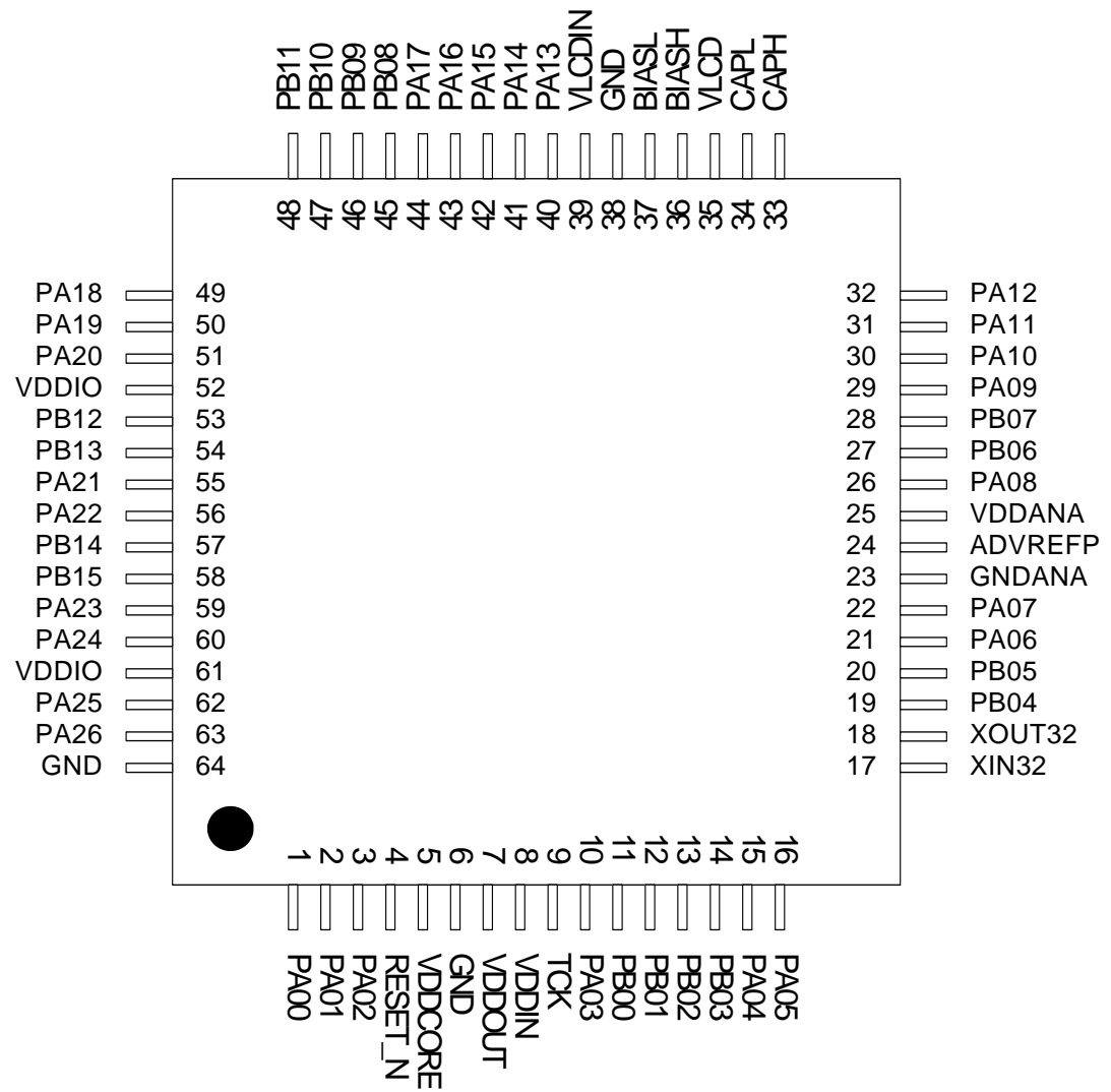
Figure 3-4. ATSAM4LC TQFP64/QFN64 Pinout
