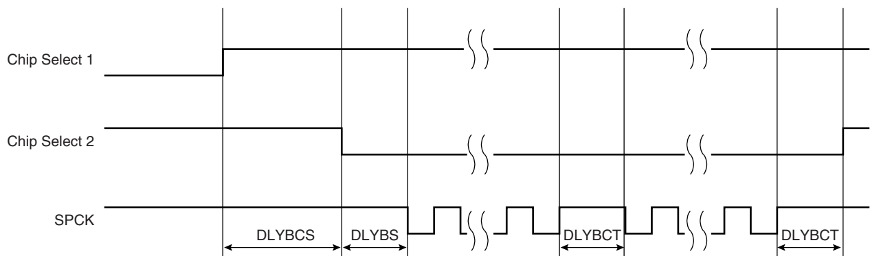
Figure 26-7. Programmable Delays
