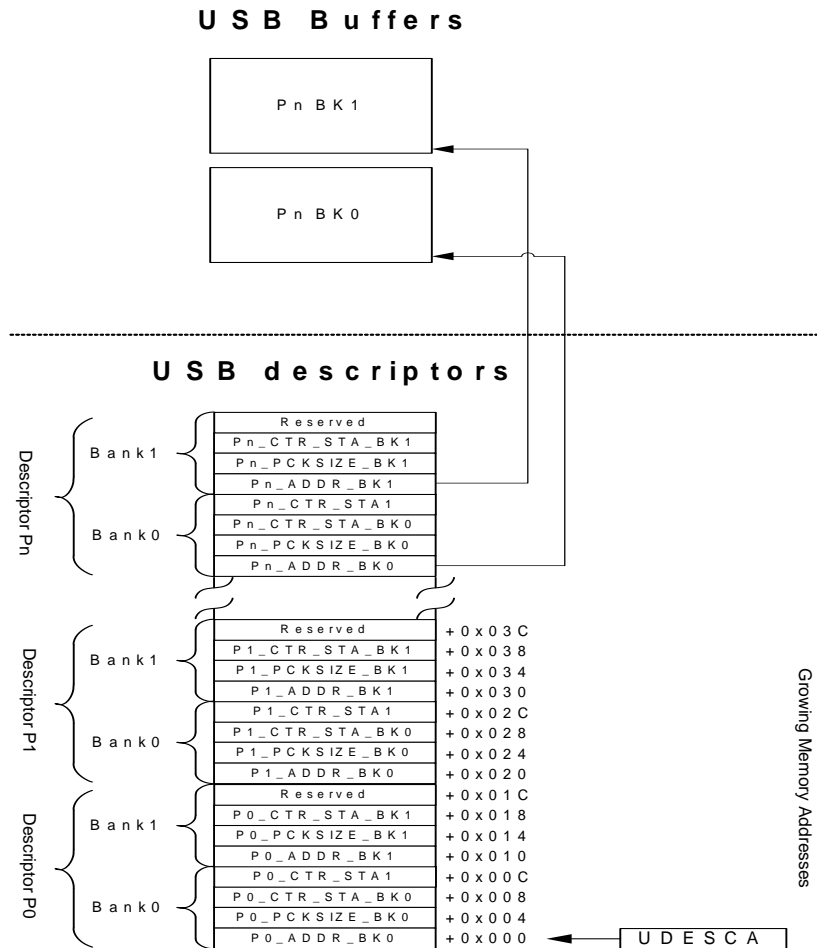
Figure 17-16. Memory organization
