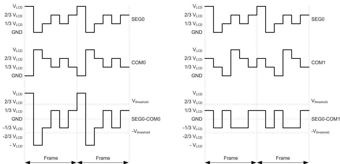
Figure 39-6. Driving a LCD With Three Common Lines
