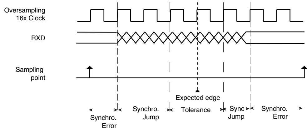
Figure 24-48. Bit Resynchronization
