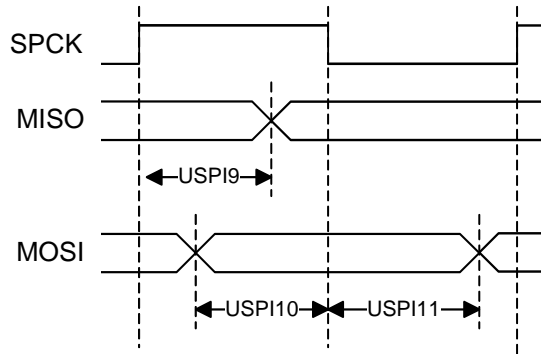
Figure 42-10. USART in SPI Slave Mode with (CPOL= CPHA= 0) or (CPOL= CPHA= 1)
