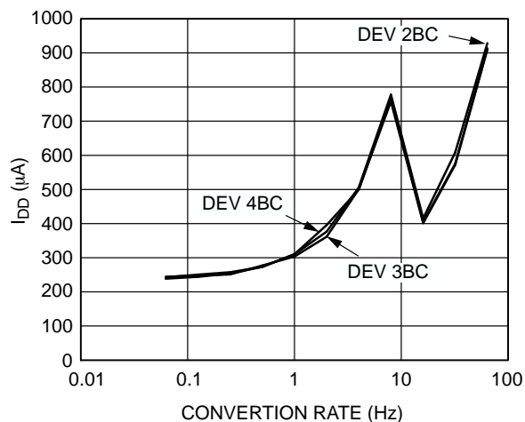
Figure 8. Operating Supply Current vs. Conversion Rate
