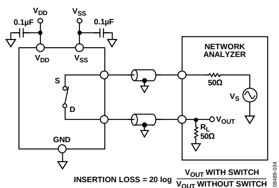
Figure 34. Bandwidth
