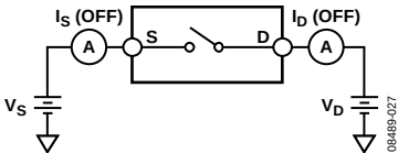
Figure 27. Off Leakage
