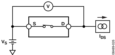
Figure 26. On Resistance
