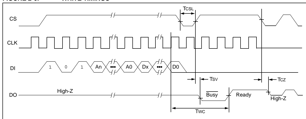
FIGURE 2-6: WRITE TIMINGS
