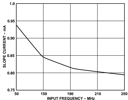
Figure 14. Slope Current, I_V , vs. Input Frequency
