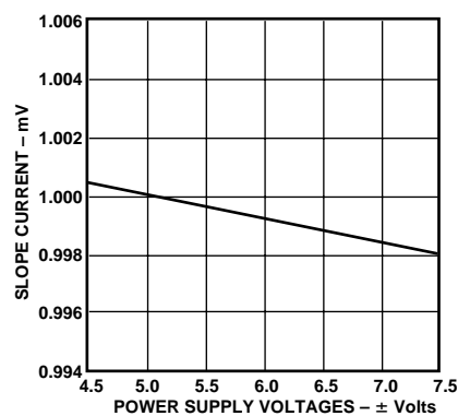
Figure 3. Slope Current, I_V , vs. Supply Voltages
