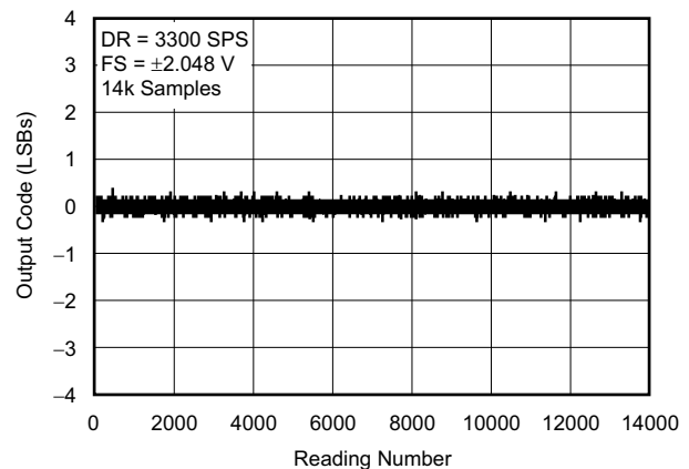
Figure 7. NOISE PLOT
