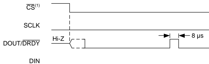
Figure 14. DOUT/ \overline{\text{DRDY}} Behavior Without Data Retrieval in Continuous Conversion Mode
